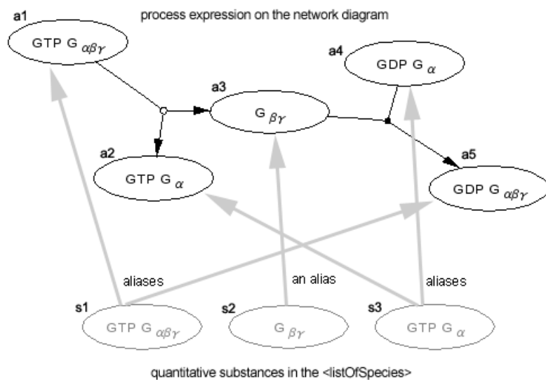
Fig. The Alias Structure of the CellDesigner
