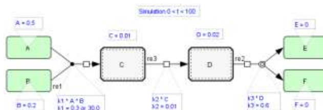
/samples/SBGNRefCard.xml
